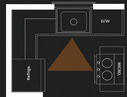
Island Kitchen
